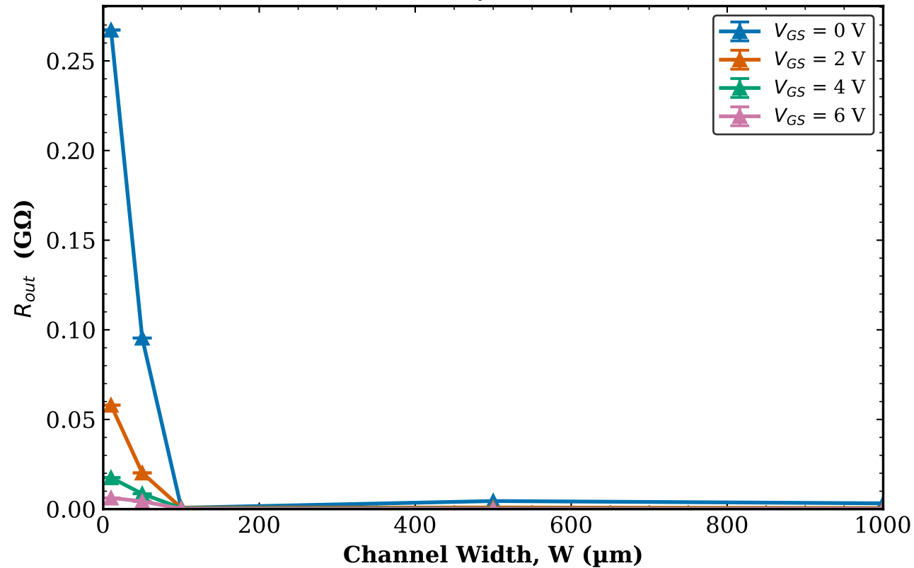
TFT1 Transistor 2 R_{out} vs W | L = 10\text{ }\mu\text{m}
